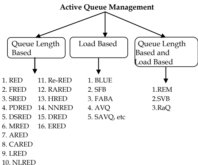
Fig 1: Classifications of existing AQM mechanisms
