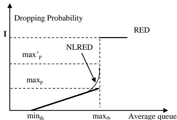
Fig 2: Comparison of packet dropping Functions for RED and NLRED [13].
